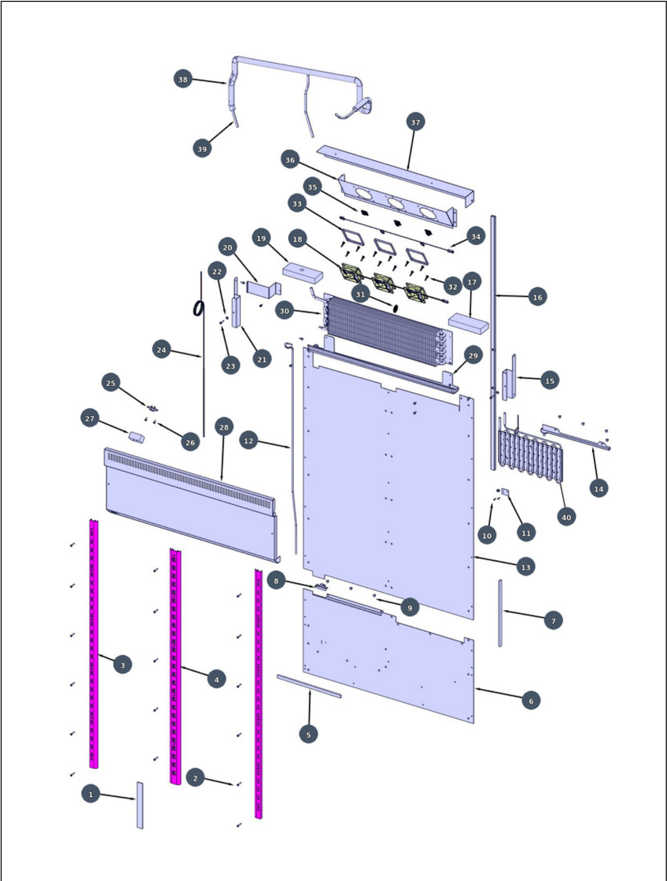
Low Side Asm View
