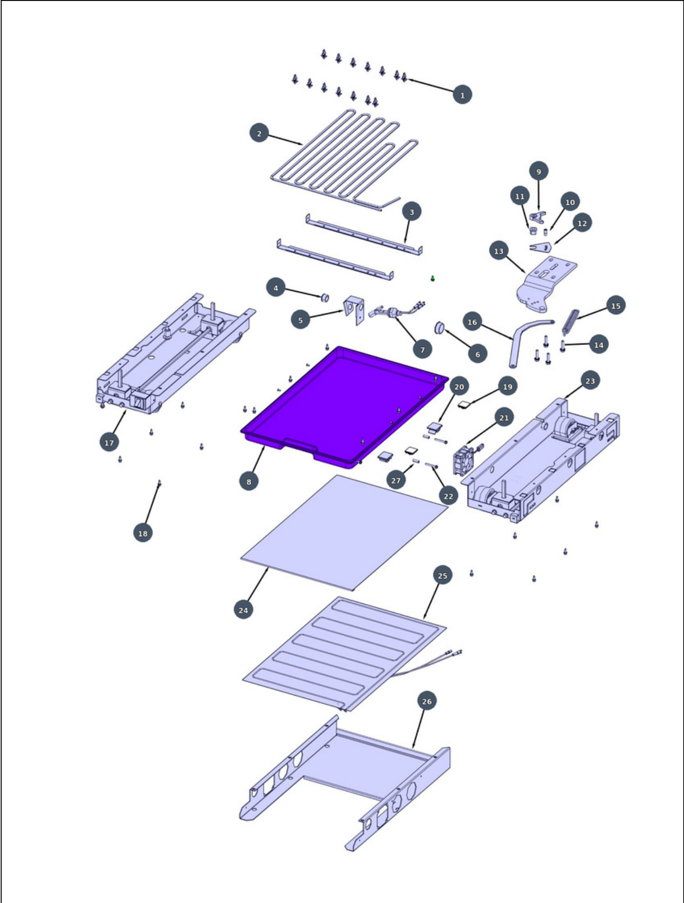
Bottom View
